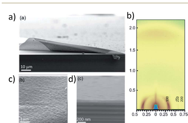
Fig. 5 (a) Highly uniform thin film of LZU-1 synthesized with in situ deprotection. (b) The crystallinity and orientation are confirmed by GIWAXS. (c) The thin film is composed of small crystallites with similar orientation and is 190 nm thick as measured by (d) cross-sectional SEM. Adapted with permission. 101 Copyright 2017 American Chemical Society.
