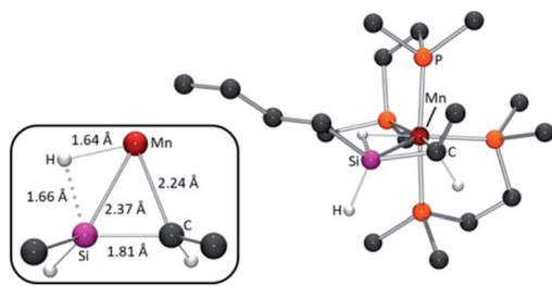
Fig. 4 Calculated structure (ball and stick diagram) for the lowest energy isomer of silene hydride complex [(\text{dmpe})_2\text{Mn}(\text{}^n\text{BuHSi}=\text{CHMe})] ( 6^{\text{Bu,H}} ). All hydrogen atoms have been omitted for clarity except those on Mn or the Si=C unit. The inset shows a top-down view of the Mn silene hydride core, with selected bond distances.
