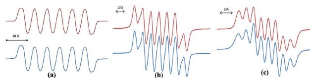
Fig. 4 Room-temperature (a) EPR spectrum of 20 simulation with ( g = 2.0055 ), a(^{27}\text{Al}) = 12.5 G; a(^{35,37}\text{Cl}) = 1.9 G; a(^{14}\text{N}) = 0.25 G; (b) EPR spectrum of compound 21 simulation with a(^{14}\text{N}) = 4.3 G, a(^{27}\text{Al}) = 8.3 G; (c) EPR spectrum of compound 22 at room temperature simulation with a(^{14}\text{N}) = 4.95 G, a(^{27}\text{Al}) = 5.2 G (Top: simulated spectrum and Bottom: experimental spectrum).
