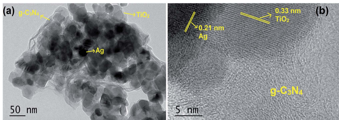
Fig. 2 (a) TEM image and (b) HRTEM image of S/Ag-TiO 2 @g-C 3 N 4 .
