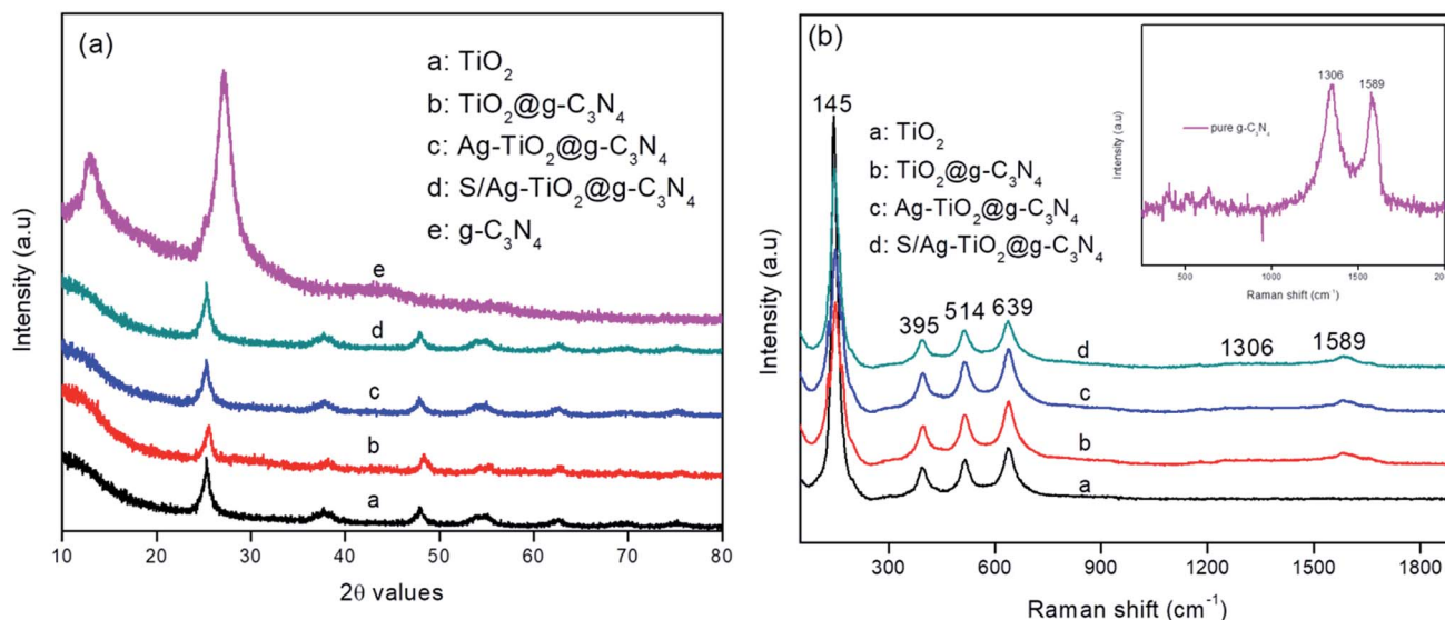
Fig. 1 (a) XRD patterns and (b) Raman spectra of the prepared composites; inset of (b) Raman spectra of pure g-C 3 N 4 .
