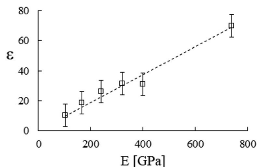
Fig. 9 Stiffness parameter versus the Young's modulus, best fitted by \varepsilon = 9.3 \times 10^{-2}E [GPa]. Data from Table 2.
