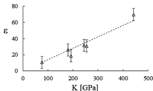
Fig. 10 Stiffness parameter versus the bulk modulus, best fitted by \varepsilon = 14.0 \times 10^{-2}K [GPa]. Data from Table 2.
