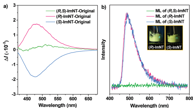
Fig. 3 CPL (a) and ML spectra (b) of the as-prepared samples of ( R,S )- ImNT , ( R )- ImNT and ( S )- ImNT under ambient conditions. The insets in (b) depict the ML images of ( R )- ImNT and ( S )- ImNT in daylight.
