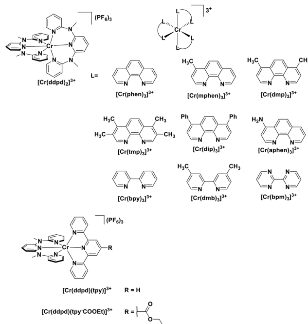
Fig. 34 Chromium(III) complexes.
