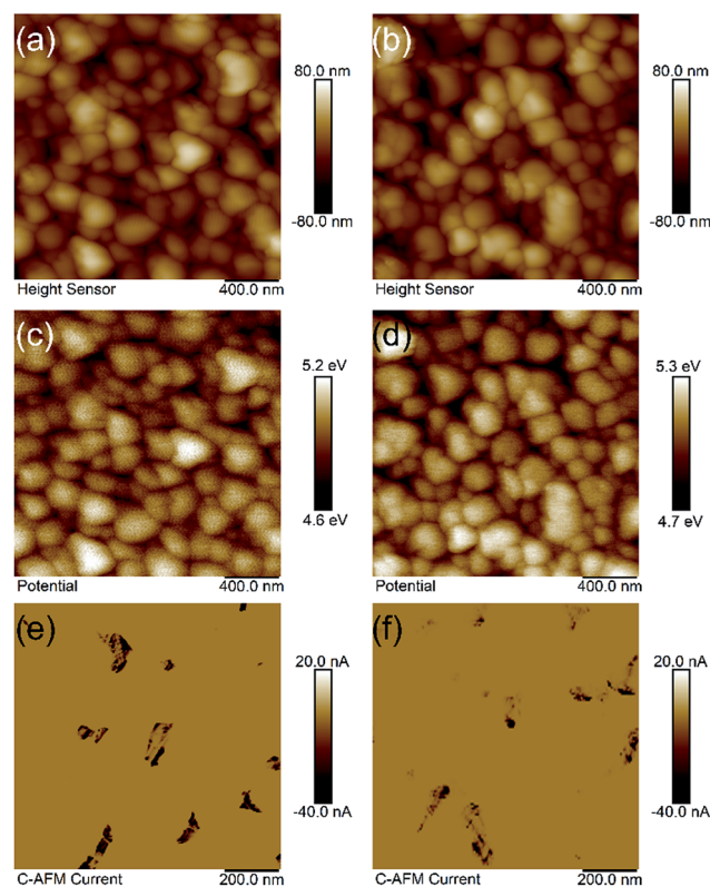
Fig. 4 (a), (c) and (e) are the height image, KPFM surface potential topology and photoconductive-AFM of the 2-Mo-BiVO 4 films; (b), (d) and (f) are the height image, KPFM surface potential topology and photoconductive AFM of the 2-Mo-BiVO 4 coated with the Fe-doped NiO catalyst. The surface potential was calibrated with an Au film (work function at 5.1 \pm 0.02 \text{ eV} ). The negative photocurrent in C-AFM corresponds to a positive charge flowing to the probe.
