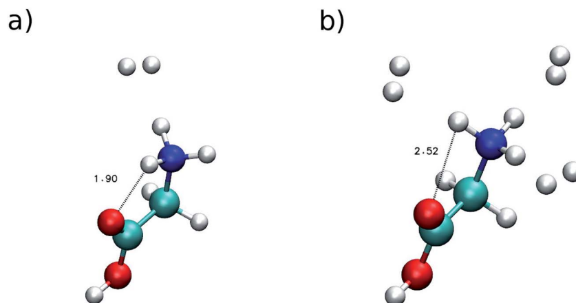
Fig. 3 Minimum configuration geometries. Panel (a) for (\text{GlyH} + \text{H}_2)^+ and (b) for (\text{GlyH} + 3\text{H}_2)^+ . Distances are in Å.
