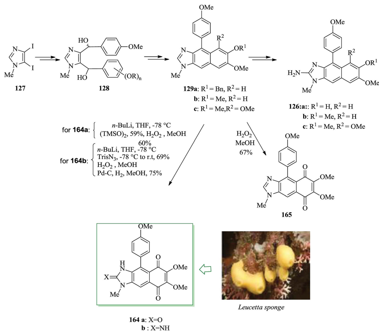
Scheme 36 Total synthesis of kealiquinone A 164a and the 2-amino congener 164b.
