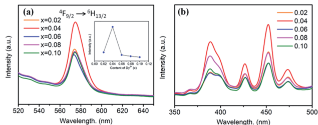
Fig. 5 (a) PL spectra (λ ex = 453 nm), inset is the dependence of the emission intensity on the Dy 3+ content. (b) PLE spectra (λ em = 573 nm) of BaTiO 3 :xDy 3+ phosphors (x = 0.02–0.10).
