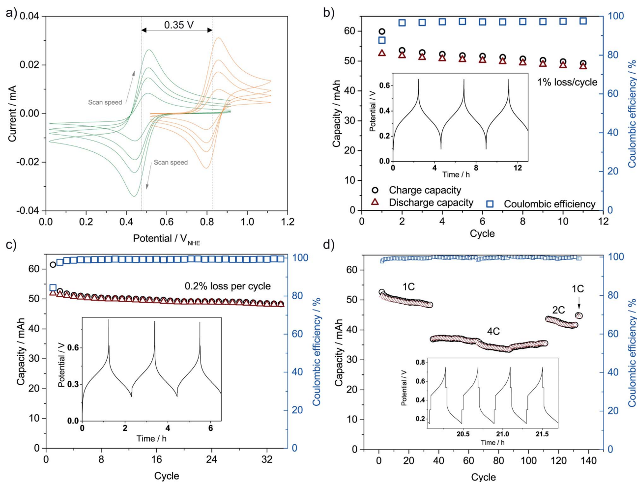
Fig. 3 (a) CVs of 2 mM solutions of K 3 Fe(CN) 6 (green) and TEMPO-sulfate (orange) in 1 M NH 4 Cl at pH 7 using a scan rate of 100, 50, 30 and 10 mV s -1 . (b) Battery cycling efficiency and capacity behaviour using 6 mL 0.4 M redox couples solutions in 1 M NH 4 Cl at pH 7 and a Nafion-117 membrane as a separator (constant current cycling at 6.1 mA cm -2 ) and (c) a Fumapem14100 membrane (constant current cycling at 12.5 mA cm -2 ). The insets show the potential–time curves of the first three cycles. (d) Coulombic efficiency and capacity behaviour by changing the current density to 12.5, 25 and 50 mA cm -2 resulting in the approximate C-rates given in the figure when continuing the experiment in (c). The inset shows the potential–time curves for four cycles at 50 mA cm -2 .
