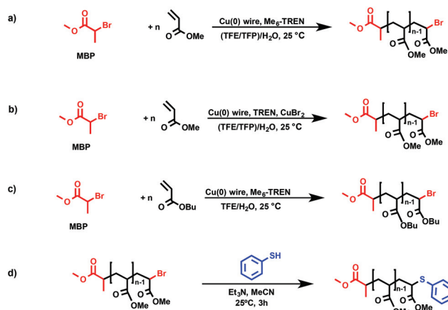
Scheme 1 (a) Me 6 -TREN and (b) TREN-mediated SET-LRP of MA in binary mixtures of TFE or TPP with water in the presence of non-activated Cu(0) wire. (c) Me 6 -TREN-mediated SET-LRP of BA in binary mixtures of TFE with water in the presence of non-activated Cu(0) wire. (d) "thio-bromo click" modification of the corresponding PMA with thiophenol.
