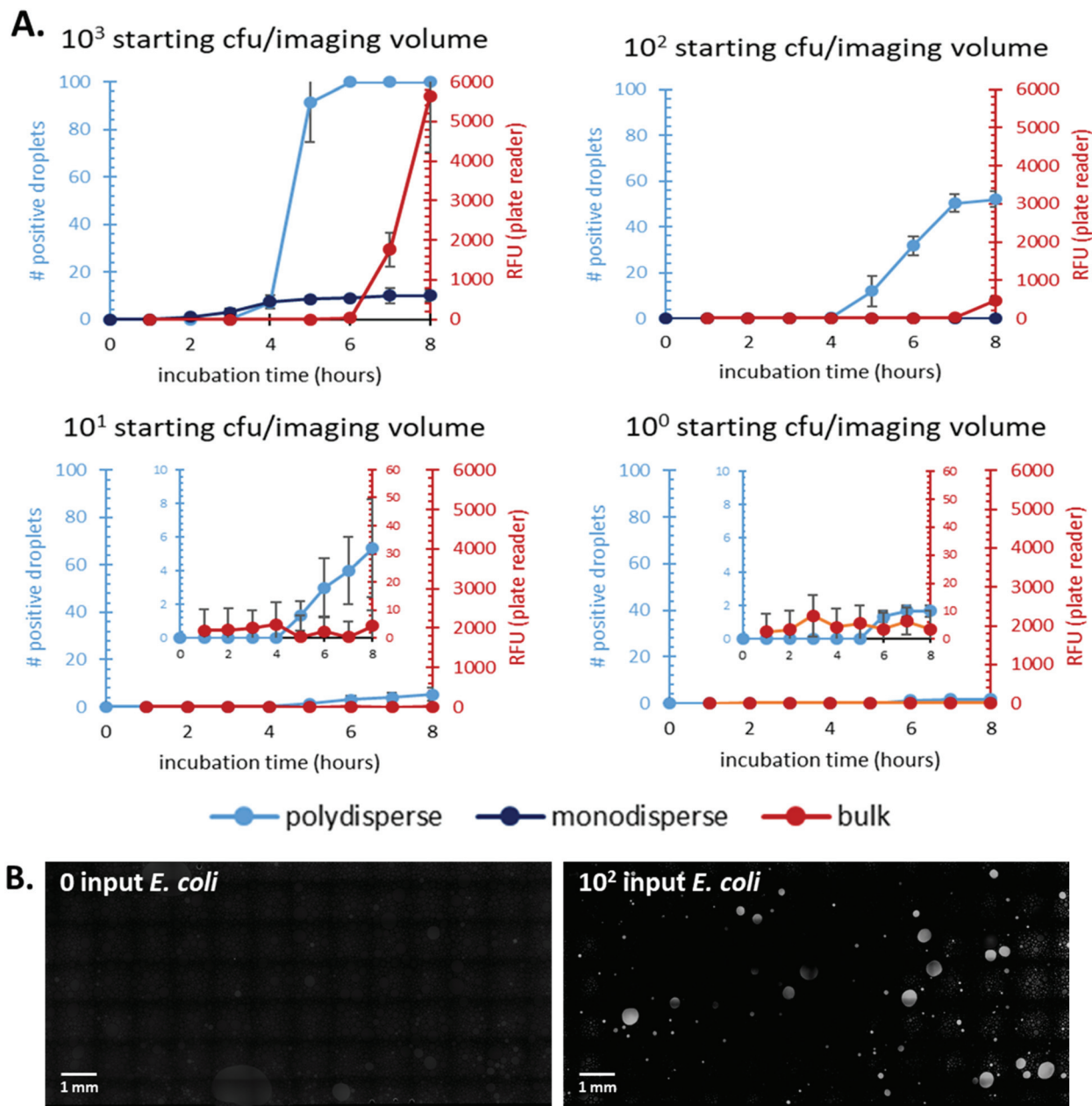
Fig. 2 Comparing E. coli cells cultured in droplets made using a droplet-forming chip (monodisperse) or our simplified method (polydisperse) to cells cultured in bulk (in well-plates). A. Time-to-detection and quantification for inputs ranging from 10^0 – 10^3 starting cfu E. coli per imaged volume. Averages of N = 3 (for polydisperse and bulk) and N = 2 (for monodisperse) are reported with error bars corresponding to \pm one standard error. The droplet-based samples (polydisperse and monodisperse) were quantified by counting the number of fluorescent droplets. B. Images post-culture of 0 and 10^2 input per 10 \mu L for polydisperse droplet samples. Images were collected and stitched together using the Nikon Ti2 software and analysed via ImageJ.
