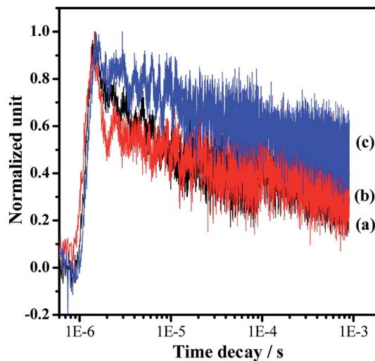
Fig. 6 Normalized transient absorption profiles of the representative samples in a vacuum: (a) Pt-Ta 3 N 5 , (b) Pt/Ba-Ta 3 N 5 and (c) Pt/Ba(0.3)-Ta 3 N 5 . The pulse laser at 355 nm was used to excite the samples for the IR tests. The cocatalyst of Pt with a loading amount of 0.5 wt% was deposited by impregnation and a subsequent H 2 reduction method.
