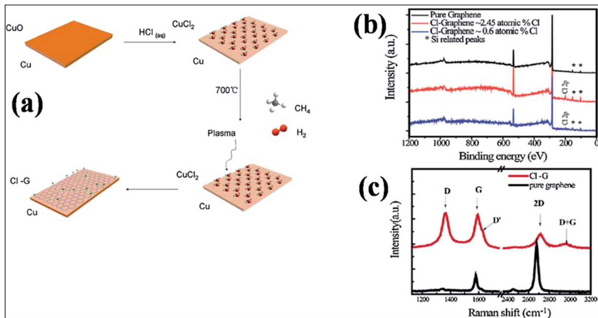
Fig. 12 (a) Schematic representation of the one-step synthesis of chlorinated mono-layer graphene: (b) XPS plots of CCl on \text{SiO}_2 compared with that of pure graphene. (c) Raman spectra of graphene (black lines) and CCl (red lines) grown on \text{SiO}_2 substrate. Reproduced with permission. 151 © 2015 Elsevier.
