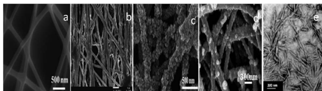
Fig. 1 SEM images of various types of CNF synthesized from cotton (a) natural electrospun CNF 56 (b) aligned CNF (scale bar 1 \mu\text{m} ) 54 (c): CdS functionalized CNF 53 (d): CeO 2 functionalized CNF 56 (e): CNF prepared by acid hydrolysis 52 (adopted with permission).
