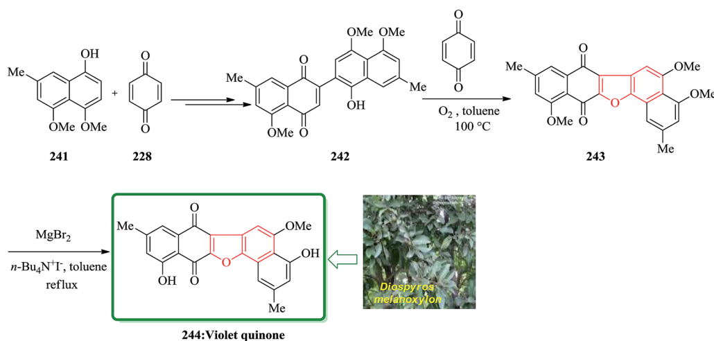
Scheme 55 Total synthesis of violet-quinone 244 .
