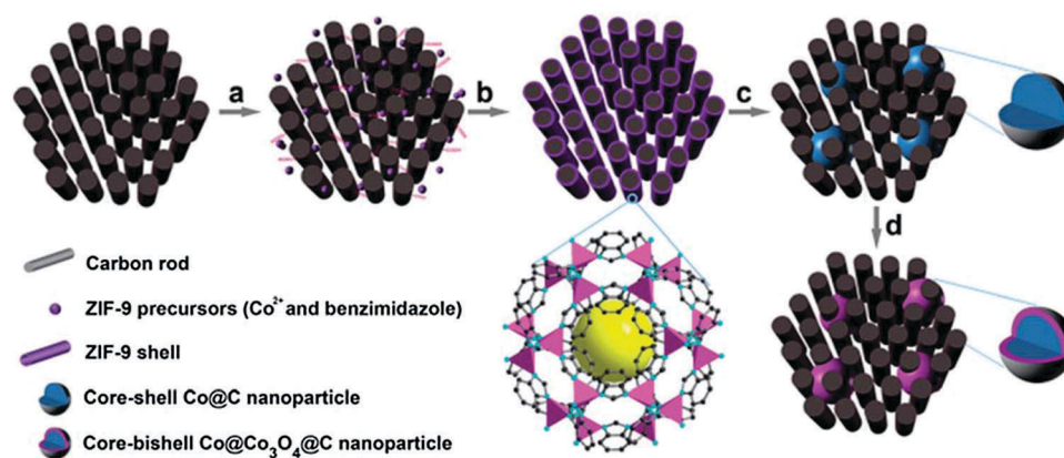
Fig. 3 Schematic illustration of the synthesis of \text{Co}@ \text{Co}_3\text{O}_4 @ \text{C}-\text{CM} : (a) functionalization of the CM with carboxylate groups, (b) growth of the MOF on the CM, (c) heat treatment under Ar flow and (d) oxidation in air at 90 °C. Reproduced from ref. 65 with permission from The Royal Society of Chemistry.
