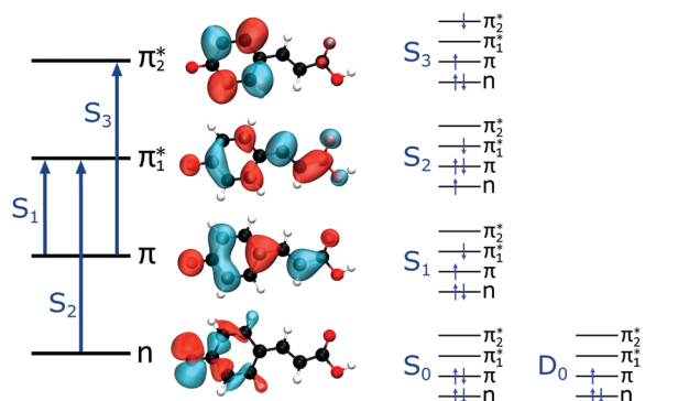
Fig. 5 Left: The main molecular orbitals involved in the transitions to the first three singlet excited states of the anion. Although the MOs plotted are calculated for p\text{CA}^- , they are similar for all the chromophores shown in Fig. 2 (see Tables S2–S5 and Fig. S3–S6, ESI†). Right: The electron configurations associated with the ground state of the anion ( S_0 ) and neutral radical ( D_0 ) and the first three singlet excited states of the anion for all the chromophores.
