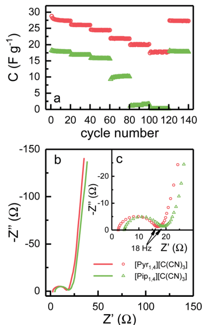
Fig. 6 (a) Specific capacitance obtained from galvanostatic charge-discharge cycling at the different rates 0.5, 1.0, 2.0, 5.0, 7.5, 10 and back to 0.5 A g -1 . (b) Nyquist plots from EIS measurements and (c) inset showing high frequency semi-circle.
