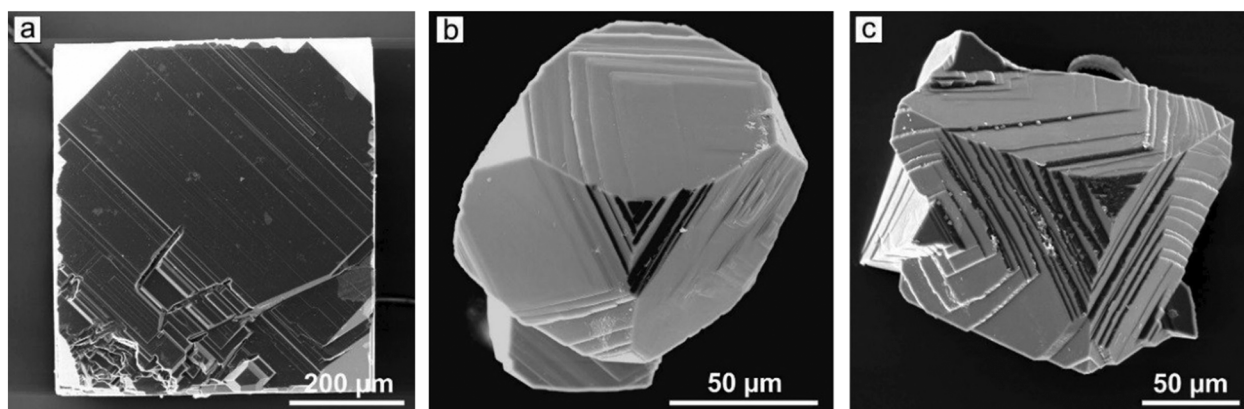
Fig. 6 SEM micrographs of diamond crystals produced in the \text{Mg-C} system: (a and b) cubic crystals; (c) cubic crystals twinned along {111}. Adapted from ref. 37 with permission from The Royal Society of Chemistry.
