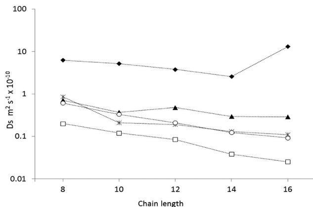
Fig. 4 A plot of the calculated diffusion coefficients from the MD simulations using experimental loadings (O), 57 MD simulations at infinite dilution 53 ( \blacktriangle ), MD simulations using more primitive models 52 ( \blacklozenge ), Hierarchical simulations 50 (*) and QENS studies 47 ( \square ). Reproduced from ref. 51 with permission from the PCCP Owner Societies.
