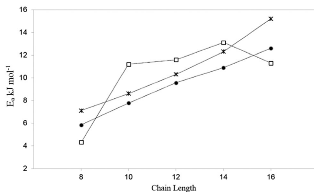
Fig. 5 A plot of the activation energy of diffusion with chain length, for the MD studies at experimental loadings ( \bullet ), 51 QENS studies 47 (*) and hierarchical simulations ( \square ). 50 Reproduced from ref. 51 with permission from the PCCP Owner Societies.
