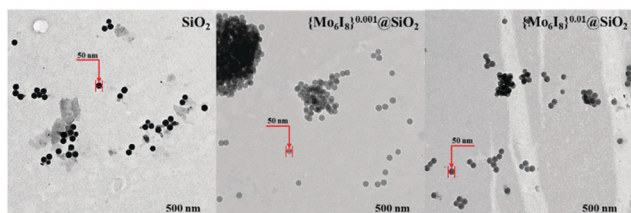
Fig. 2 TEM images of neat \text{SiO}_2 and \{\text{Mo}_6\text{I}_8\}@SiO_2 NPs.
