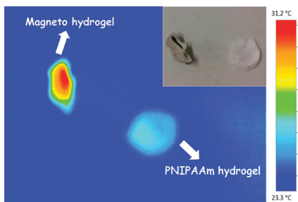
Fig. 5 Thermal images of magneto-hydrogel and reference material without MNP after 1 minute of AMF exposure ( I = 15.6 A, f = 745 kHz, H \sim 20 kA m -1 ); inset shows photographs of the samples.
