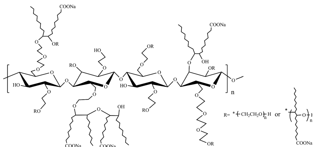
Fig. 1 Structure of epoxidized soybean oil modified hydroxyethyl cellulose polymeric surfactant.
