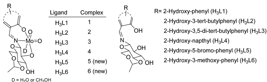
Fig. 1 cis -Dioxo molybdenum(vi) complexes of H 3 Ln.
