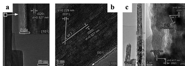
Fig. 3 (a) Low-magnification TEM image of a single β-FeOOH nanorod viewed along the [101] direction. The insert HRTEM image indicates that the nanorod exposes the {010} planes. (b) Another HRTEM image viewed along the [100] orientation, also showing the preferential exposure of the {010} planes, (c) low- and high-magnification TEM images of a single γ-Fe 2 O 3 nanorod, indicating the dominant exposure of the {110} and {001} planes (modified with permission from ref. 39, copyright 2012 Wiley-VCH).
