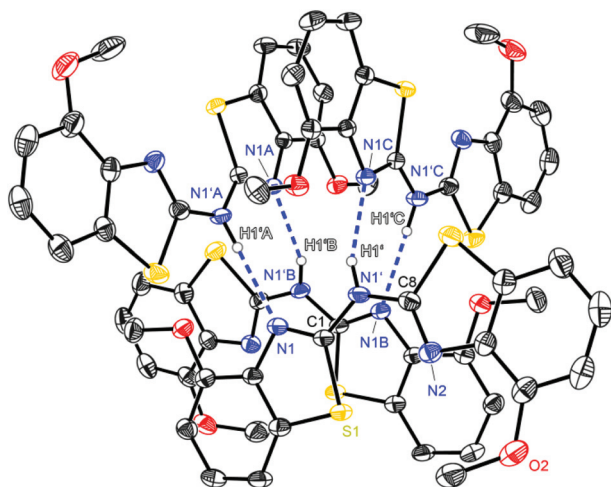
Fig. 4 Molecular structure of a hydrogen bridged tetramer of (4-OMeNCSC 6 H 3 ) 2 NH ( 3 ). Anisotropic displacement parameters are depicted at the 50% probability level. C–H hydrogen atoms are omitted for clarity. Structural data are given in Tables 1–3.
