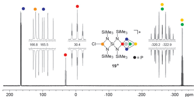
Fig. 3 ^{31}\text{P}\{^1\text{H}\} NMR spectrum of 19[\text{GaCl}_4] ( \text{CD}_2\text{Cl}_2 , r.t.); insets show experimental (upwards) and fitted spectra (downwards); \text{A}_2\text{MX}_2 spin system of 19^+ : \delta(\text{P}_\text{A}) = -322.9 ppm, \delta(\text{P}_\text{B}) = -320.2 ppm, \delta(\text{P}_\text{M}) = 30.4 ppm, \delta(\text{P}_\text{X}) = 165.5 ppm, \delta(\text{P}_\text{Y}) = 166.8 ppm, ^1J(\text{P}_\text{A}\text{P}_\text{B}) = -189.8 Hz, ^1J(\text{P}_\text{A}\text{P}_\text{X}) = -143.4 Hz, ^1J(\text{P}_\text{B}\text{P}_\text{X}) = -147.7 Hz, ^1J(\text{P}_\text{M}\text{P}_\text{X}) = -245.1 Hz, ^2J(\text{P}_\text{A}\text{P}_\text{M}) = 18.8 Hz, ^2J(\text{P}_\text{B}\text{P}_\text{M}) = 18.0 Hz.
