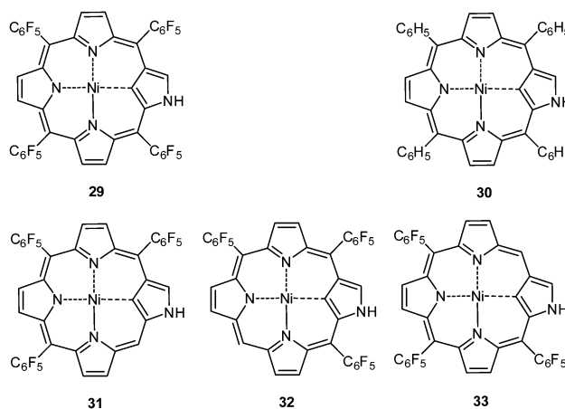
Fig. 16 Molecular structures of the N-confused porphyrin receptors 29–33 as used in the studies of Maeda et al. 39
