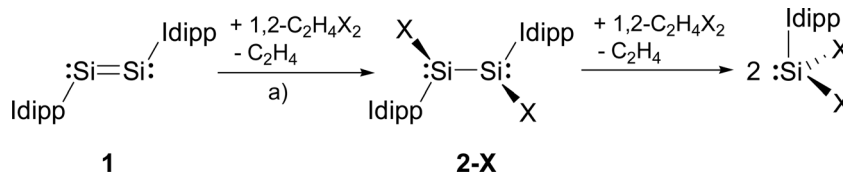
Scheme 1 Synthesis of the Si(I) halides 2-X ( X = \text{Cl, Br, I} ) and further oxidation to the Si(II) halides \text{SiX}_2(\text{Idipp}) ( \text{Idipp} = \text{C}[\text{N}(\text{dipp})\text{CH}_2]_2 ); a) X = \text{Cl} : toluene, -30^\circ\text{C} ; X = \text{Br} : toluene, -45^\circ\text{C} ; X = \text{I} : THF, -70^\circ\text{C} . Formal charges are not included for simplicity.
