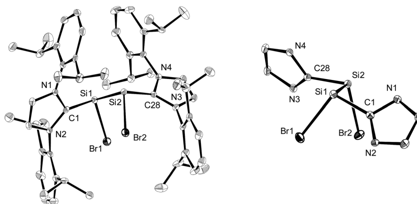
Fig. 1 Left: Diamond plot of the molecular structure of 2-Br · 0.5( n\text{-C}_6\text{H}_{14} ) in the single crystal. The thermal ellipsoids are set at 30% probability at 123(2) K, and the hydrogen atoms and n -hexane molecules are omitted for clarity. Right: View of the 2-Br molecule along the Si–Si bond axis illustrating the synclinal arrangement of the Br atoms and the antiperiplanar orientation of the NHC groups (N-bonded dipp substituents are omitted for clarity). Selected bond lengths [Å], bond angles [ ^\circ ] and torsion angles [ ^\circ ] for 2-Br · 0.5( n\text{-C}_6\text{H}_{14} ): C1–Si1 1.940(3), Si1–Br1 2.3602(8), Si1–Si2 2.385(1), Si2–Br2 2.3677(9), Si2–C28 1.936(3); C1–Si1–Br1 102.22(9), C1–Si1–Si2 97.87(9), Br1–Si1–Si2 103.78(4), Si1–Si2–Br2 104.17(4), Si1–Si2–C28 96.74(9), Br2–Si2–C28 101.42(9); C1–Si1–Si2–C28 161.5(1), Br1–Si1–Si2–Br2 -46.81(4) .
