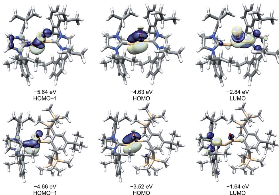
Fig. 6 Selected Kohn–Sham orbitals (B97-D3/I) of \mathbf{3}_{\text{calc}} (top) and (Z)\text{-(SiIdipp)Si}=\text{Si}(\text{Br})\text{R} (bottom, \text{R} = \text{C}_6\text{H}_2-2,6-\{\text{CH}(\text{SiMe}_3)_2\}_2-4-t\text{Bu} ) and their corresponding energy eigenvalues. Isosurface value: 0.05 \text{ e bohr}^{-3} . The LUMO of \mathbf{3}_{\text{calc}} is a symmetrical combination of a \pi^* NHC and \sigma^* Si–I orbital, whereas the LUMO of (Z)\text{-(SiIdipp)Si}=\text{Si}(\text{Br})\text{R} is a \pi^* NHC orbital.
