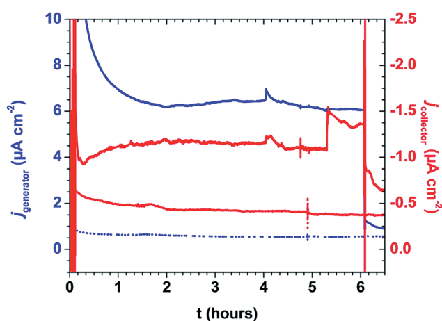
Fig. 7 Current-time traces for \text{nanoTiO}_2|\text{RuP}^{2+}(10\text{-AO})|-\text{RuCP}(\text{OH})_2^{2+}(10\text{-AO}) E_{\text{gen}} = 0.64 V and E_{\text{coll}} = -0.61 V under illumination. Blue traces (left axis) indicate generator current under illumination (solid) and in the dark (dotted) while red traces (right axis) indicate collector current with the same convention. Cathodic current arises from \text{O}_2 reduction at the FTO collector electrode (conditions: \sim 200 \text{mW cm}^{-2} white light illumination; 400 nm long-pass filter; pH 8.8 , 0.1 M \text{H}_2\text{PO}_4^-/\text{HPO}_4^{2-} ; 0.4 M \text{NaClO}_4 ; ref = SCE; Aux = Pt-mesh).
