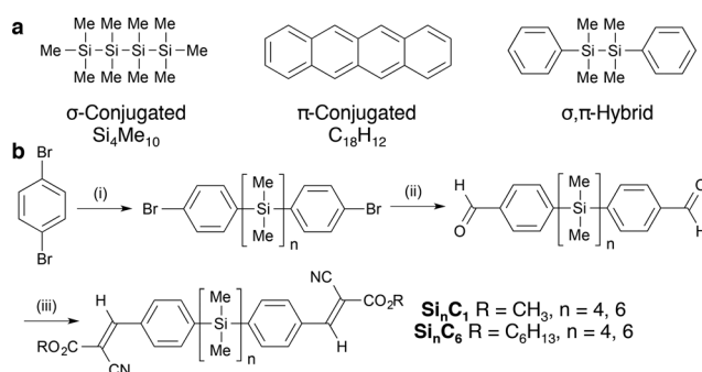
Fig. 1 (a) Representative \sigma -conjugated, \pi -conjugated and hybrid materials. (b) Synthesis of cyanovinylsilanes. (i) n\text{-BuLi} , \text{Et}_2\text{O} , 0^\circ\text{C} ; \text{Cl(SiMe}_2)_n\text{Cl} (82–96%). (ii) n\text{-BuLi} , \text{Et}_2\text{O} , 0^\circ\text{C} ; DMF, (iii) \text{RO}_2\text{CCH}_2\text{CN} , piperidine, benzene, 80^\circ\text{C} (72–89%, 2 steps).
