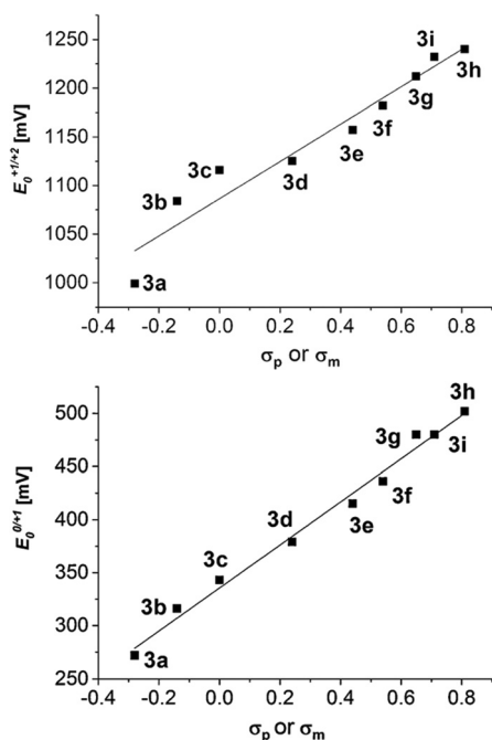
Fig. 2 Linear correlation plots of the first oxidation potentials E_0^{0/+1} [mV] (bottom) and second oxidation potentials E_0^{1/2+2} [mV] (top) of 2,6-diaryl-substituted dithienothiazines 3a–i against Hammett \sigma_p or \sigma_m parameters ( E_0^{0/+1} = 201\sigma_{p/m} + 336 [mV], r^2 = 0.9889 ; E_0^{1/2+2} = 192\sigma_{p/m} + 1086 [mV], r^2 = 0.9406 ).
