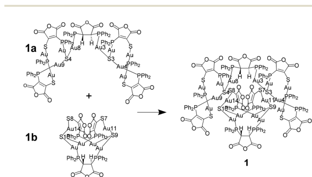
Scheme 2 Formal division of compound 1 into its two neutral subunits under specification of according total energies, summing up to E = -649.5 \text{ kJ mol}^{-1} .
