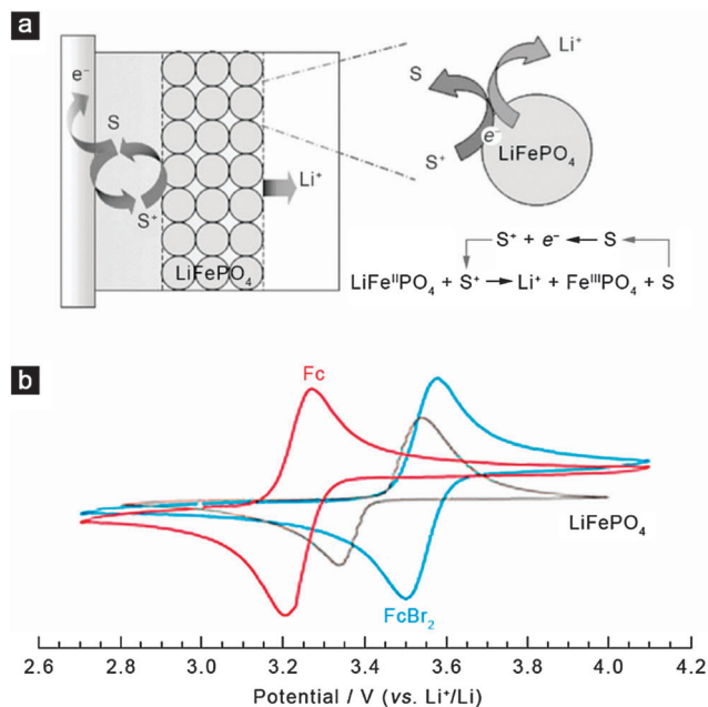
Fig. 14 (a) The principle of redox targeting of an insulating electrode material such as LiFePO 4 by a freely diffusing molecular shuttle S. Upon charging, the molecular shuttle is oxidized into S + at the current collector, and delivers the charge to the solid particles LiFePO 4 . S + will be reduced back to S if the redox potential matches the Fermi level of LiFePO 4 . During this process, Fe II is oxidized into Fe III , and Li + ions will be released. Upon discharge, S + is reduced at the current collector to S so electrons can be delivered to FePO 4 to form LiFePO 4 with the simultaneous immigration of Li + ions. Reproduced with permission from ref. 125. Copyright 2006, Wiley. (b) Cyclic voltammograms of the redox shuttles Fc and FcBr 2 , as well as a cathodic Li + -storage material LiFePO 4 . Reproduced with permission from ref. 124. Copyright 2013, Royal Society of Chemistry.
