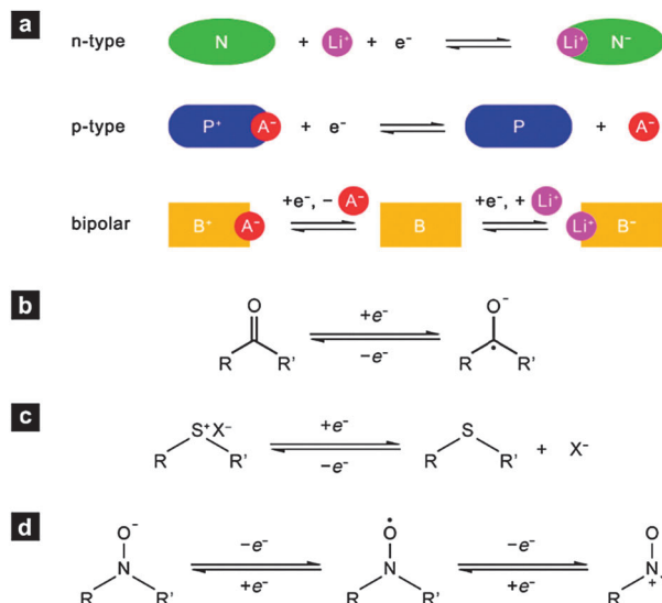
Fig. 18 (a) Redox reaction of n-type (N), p-type (P) and bipolar (B) redox-active organics and metalloorganics. \text{A}^- stands for anion of the electrolyte. Reproduced with permission from ref. 170. Copyright 2013, Royal Society of Chemistry. Corresponding redox mechanism for redox-active organics: (b) carbonyl compounds, (c) thioethers, and (d) organic free radical compounds.
