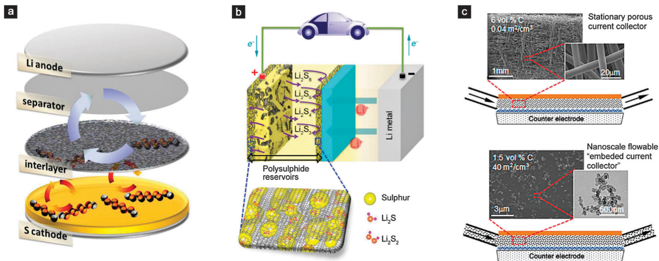
Fig. 17 Electrode architectures for polysulphide-based Li-redox flow cells. (a) Bi-functional interlayer electrode architecture. Reproduced with permission from ref. 150. Copyright 2014, American Chemical Society. (b) Compound-sandwiched electrode architecture. Reproduced with permission from ref. 167. Copyright 2014, Wiley. (c) Conventional flow cell architecture using stationary carbon fibre current collector (top) and nanoscale flowable "embedded current collector" (bottom) providing electronically conductive flowing redox electrodes based on nanoscale percolating networks of carbon black particles. Reproduced with permission from ref. 168. Copyright 2014, American Chemical Society.
