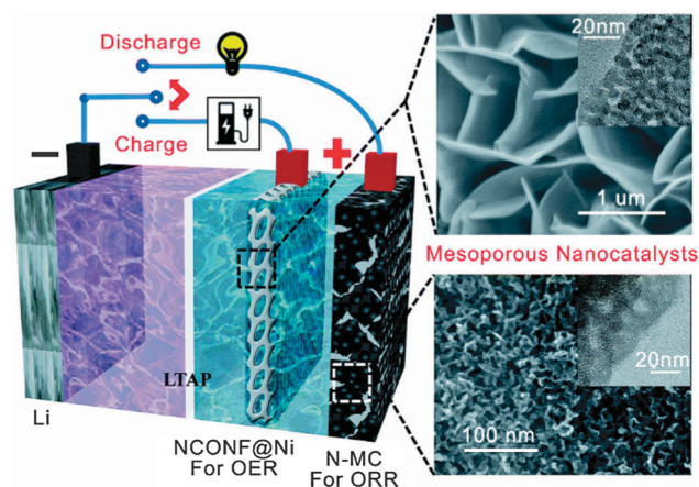
Fig. 9 Schematic of the decoupled electrodes loaded with mesoporous nanocatalysts. The upper-right SEM and TEM images showing the mesoporous NiCo 2 O 4 nanoflakes directly grown onto nickel foam (NCONF@Ni) as the OER catalyst; the lower right SEM and TEM images shows the N-doped mesoporous carbon (N-MC) as the ORR catalyst. Reproduced with permission from ref. 86, Copyright 2014 Royal Society of Chemistry.
