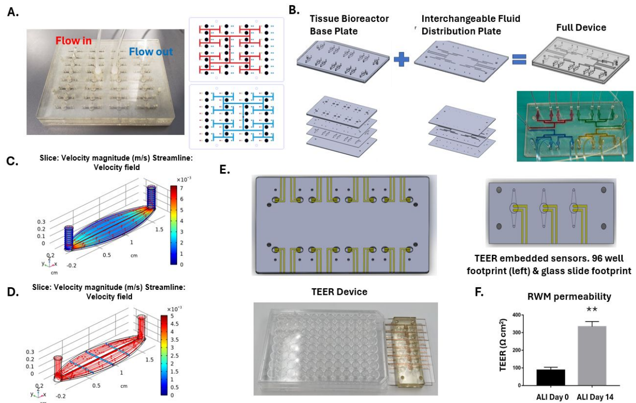
Figure 2. Multiplex fluid distributor and TEER sensor design and validation. A. The image of the fluid distribution layer and the design (For a 32-unit device). Fabricated multiplexed plate with fluid distribution layer connecting the inlets and outlets of the bottom channels. Red-bottom inlet, blue-bottom outlet. B. Fabrication of the MPS with interchangeable fluid distribution plate (for a 16-unit device) and validation of the fluid distribution using 4 different colors, allowing for 4 different experiments with 4 replicates simultaneously. (C) The 3D COMSOL model demonstrated the xy-cross section of the microfluidic device, indicating homogeneous flow. (D) Similarly, the yz-cross section showed that the flow is stronger in the middle of the channel, reaching a speed of 0.005 m/s, while the flow at the surface is slower, with a speed of 0.001 m/s. E. TEER sensor design and image. F. RWM permeability measured using the integrated TEER from Day 0 to Day 14 in the air-liquid interface (ALI) culture.
