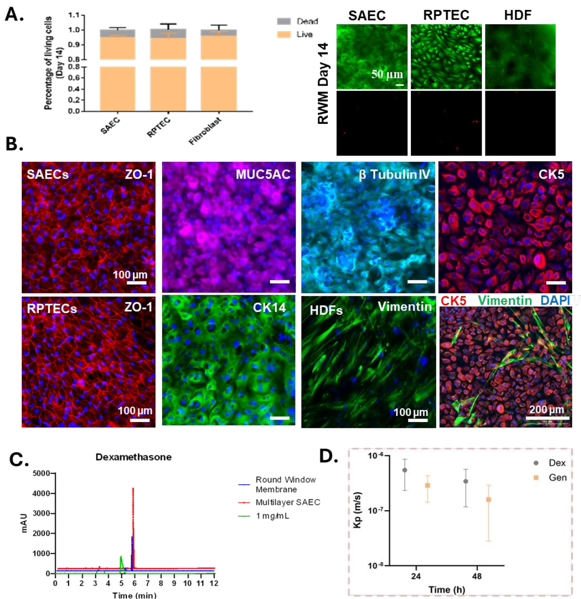
Figure 3. Characterization of the RWM cell model and RWM drug delivery. A. Live & dead assay - cell viability (left: quantitative analysis of individual RWM cell types in co-culture; right: images of cell viability. Green- live cells, red- dead cells). B. IF staining (each cell layer) - key marker expression 14 days post ALI culture. SAEC was characterized by ZO-1, MUC5AC, beta-tubulin IV, and CK5; RPTEC was characterized by ZO-1 and CK14; HDF was characterized by vimentin. The lower-right image displays a projection of HDF cells cultured beneath the SAEC layer. C. Drug diffusion across the RWM barrier (LC-MS/MS) indicated a shift of peaks in the chromatogram in the presence of RWM cell type (blue: 3 cell layer, red: SAEC mucosal cell layer
