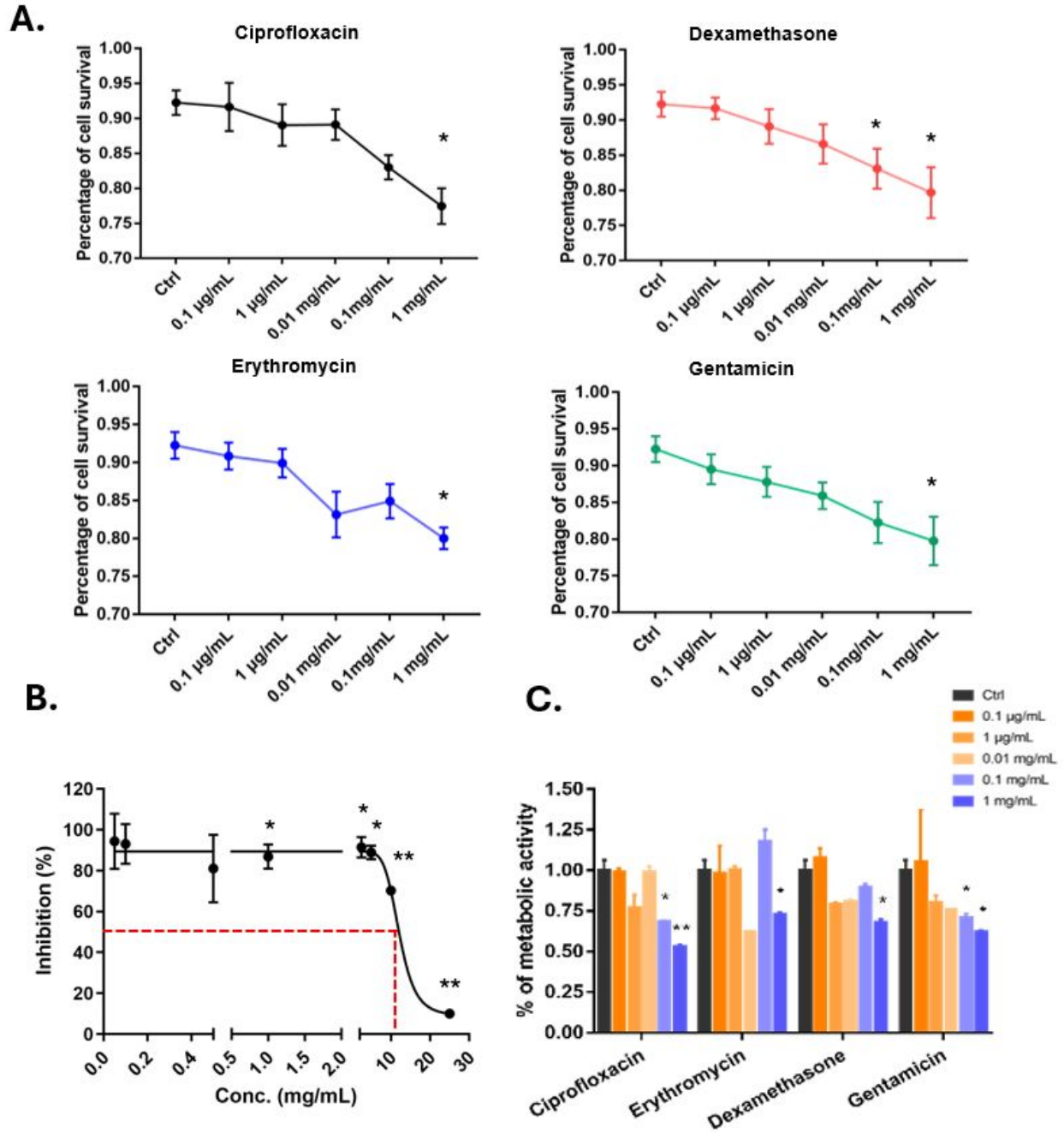
Figure 4. Cellular drug response in RWM model. A. Live/dead assay – cell viability in the presence of drugs in various doses; B. TD_{50} analysis of drug-ciprofloxacin; C. LDH assay-membrane integrity in the presence of drugs. Statistical significance was determined using Student's t-test for pairwise comparisons between each treated group and its control group. p-
