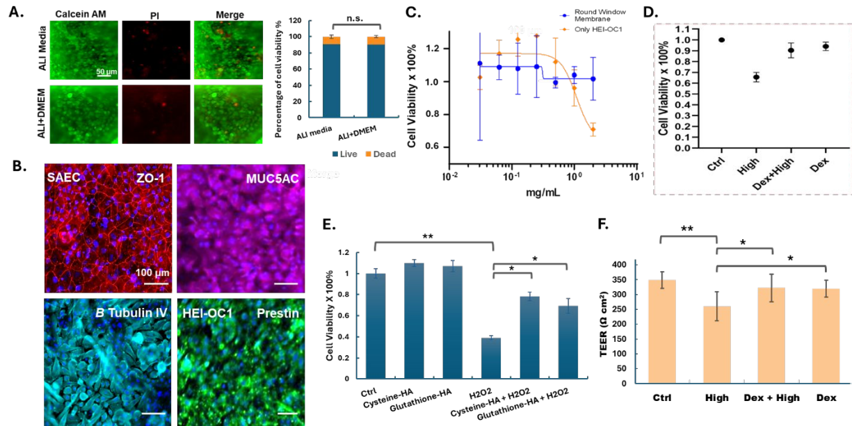
Figure 5. Characterization of the coculture platform – RWM + sensory epithelial compartment (HEI-OC1 cells) and drug screening. A. Live/dead staining assay - hair cell viability in co-culture, in two different media (Pneumatic-ALI-S alone or ALI-S + DMEM with 10% FBS). B. IF staining – hair cell/SAEC key marker expressions. C. Dexamethasone toxicity: dose response curve – anti-inflammatory drug toxicity to hair cells, with and without RWM cell types. D. Hair cell response: ototoxic injury model using acute inflammation and assessing hear-loss preventive drugs responses. Proinflammatory cytokine cocktail treatment (High), dexamethasone alone (Dex) (0.5 mg/mL) or co-treatment of dexamethasone and the proinflammatory cytokine cocktails (Dex + High), RWM/cochlear cell coculture without treatment (Ctrl). E. Hair cell response: ototoxic injury model using excessive oxygen species and assessing hear-loss preventive drugs responses. F. Analysis of barrier function using the integrated TEER sensor in the ototoxicity model and dexamethasone treatment. Proinflammatory cytokine cocktail treatment (High), dexamethasone alone (Dex) (0.5 mg/mL) or co-treatment of dexamethasone and the proinflammatory cytokine cocktails (Dex + High), RWM/cochlear cell coculture without treatment (Ctrl).
