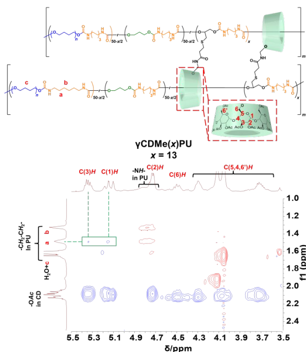
Fig. 2. 600 MHz 2D NOESY NMR spectrum of \gamma CDMe(13)PU in chloroform- d . The NOE correlation signals between the TAc y CD units and the PU main chains are highlighted.
