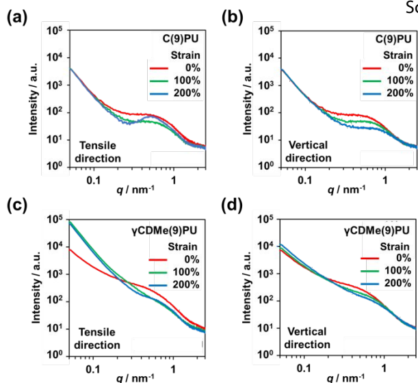
Fig. 7. SAXS profiles of C(9)PU with 0%, 100% and 200% strains in the (a) tensile and (b) vertical directions. SAXS profiles of \gamma CDMe(9)PU with 0%, 100% and 200% strains in the (c) tensile and (d) vertical directions.
