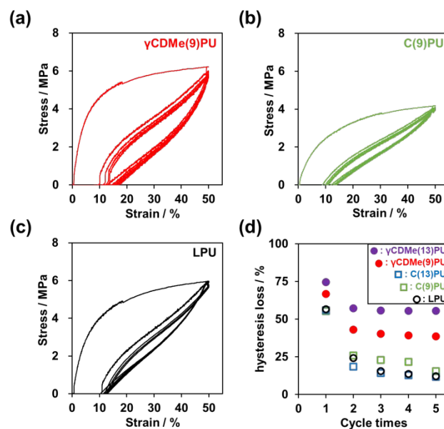
Fig. 4. The cyclic stress–strain curve with fixed strain (50%) of (a) \gamma CDMe(9)PU, (b) C(9)PU and (c) LPU. (d) Hysteresis loss calculated from the cyclic stress–strain curve. The cycles were performed five times.
