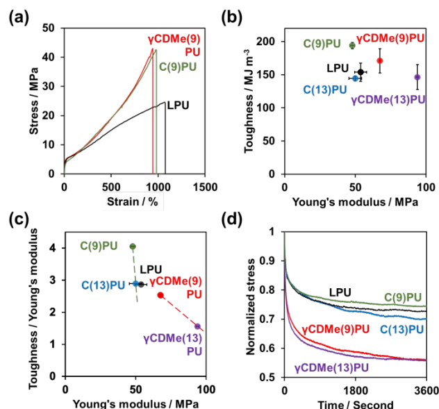
Fig. 3. (a) Stress–strain curves, (b) plots of toughness versus Young's modulus, (c) plots of toughness divided by Young's modulus and Young's modulus, and (d) relaxation time curves of LPU, \gamma CDMe( x )PU and C( x )PU. The \gamma CDMe( x )PU showed higher fracture stress, Young's modulus and shorter relaxation times than the LPU and C( x )PU.
