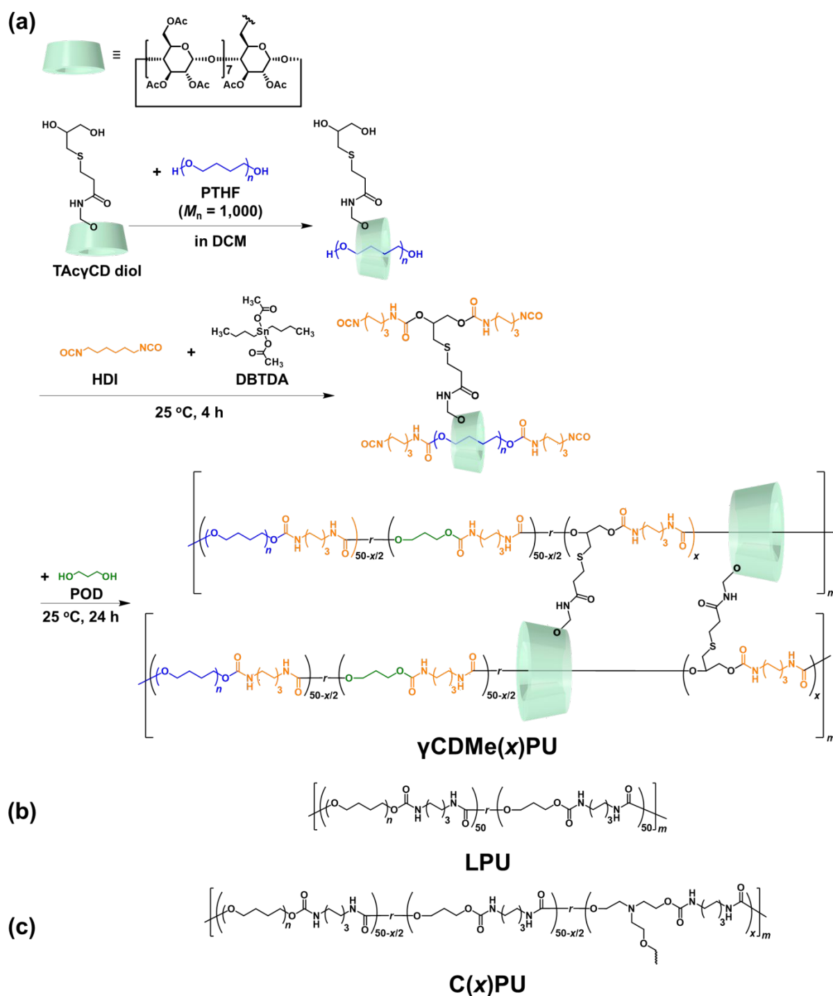
Fig. 1. (a) Synthesis of \gamma CDMe(x)PU and chemical structures of (b) LPU and (c) C(x)PU, where x refers to the molar ratio of TAcycD diol monomer or TEA monomer.
