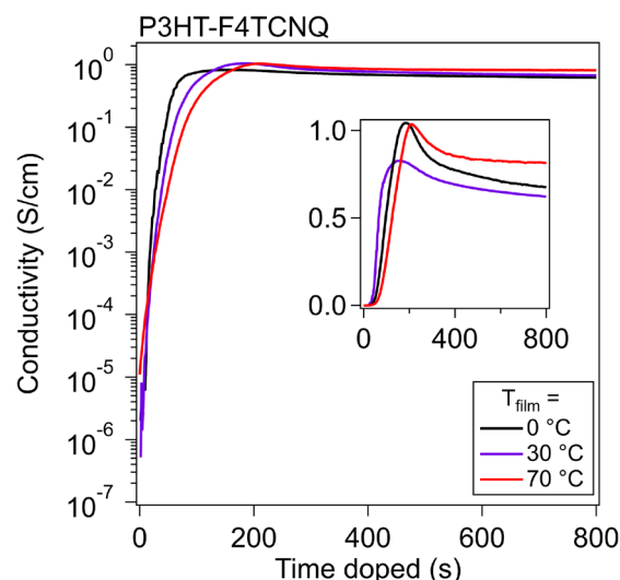
Figure 2. In situ conductivity curves of F4TCNQ-doped P3HT.
