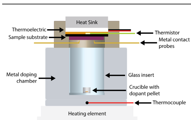
Figure 1. Cross section of apparatus for vapor doping experiments. Metal doping chamber houses glass insert with alumina crucible and F4TCNQ pellet within. F4TCNQ pellet is vaporized by heating the metal doping chamber to a desired temperature on a hot plate, whose temperature is monitored by a thermocouple in the base. The sample is simultaneously measured and held stable by the metal contact probes, and a thermoelectric holds the temperature of the sample to a set constant from 0 °C to 70 °C. All vapor doping experiments were performed in an argon glovebox.
