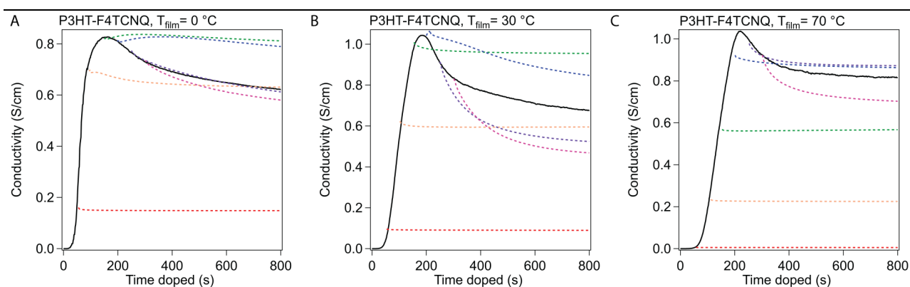
Figure 3. Stabilization of \sigma at 50 s intervals. Samples of F4TCNQ-doped P3HT were taken off the dopant (“curtailed”) at 50 s intervals as to replicate the conditions of samples that were taken off at that time for other experiments, such as UV-Vis, Raman spectroscopy, and grazing incidence wide angle x-ray scattering. The dotted line indicates the shape of the \sigma curve when the sample is taken off at the beginning of the dotted line (i.e. the red dotted line was curtailed at 50 s). The solid line indicates the curve of \sigma when doping is not curtailed.
