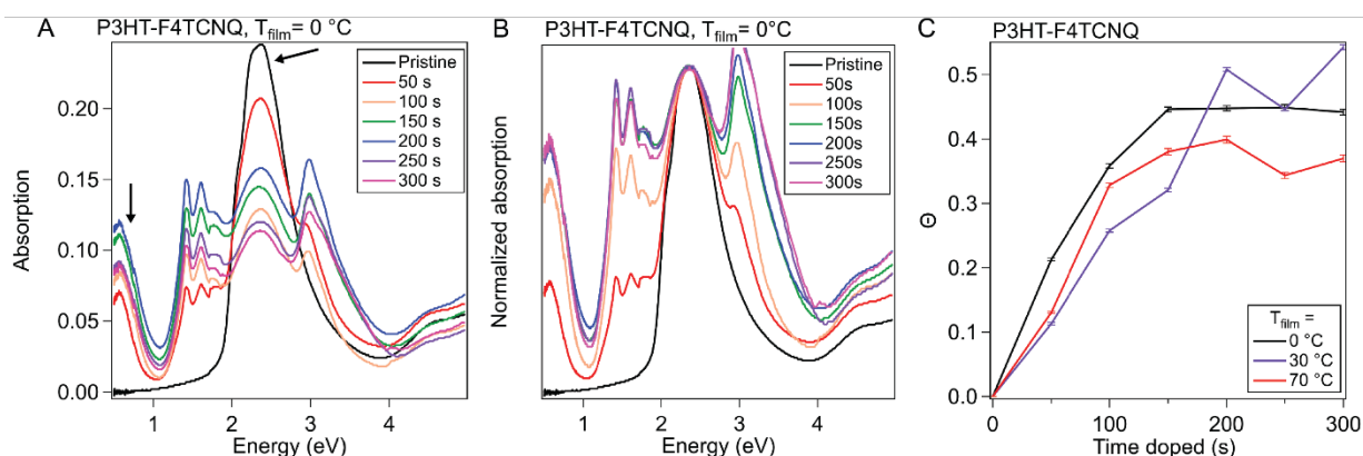
Figure 4. UV-Vis-NIR Absorption of P3HT and P3HT-F4TCNQ samples. (A) Representative absorption spectra of P3HT-F4TCNQ films doped to the levels shown in figure 3 (0 s to 300 s at 50 s intervals), with sample temperature 0^\circ\text{C} , shown normalized to the neutral P3HT peak at 2.3 eV in (B). The peak at 0.5 eV is attributed to the polaron and the peak at 2.3 eV is attributed to the neutral P3HT. (C) Plotting the fraction of doped P3HT sites ( \Theta ) versus the doping time. The value of \Theta is correlated to charge carrier concentration.
