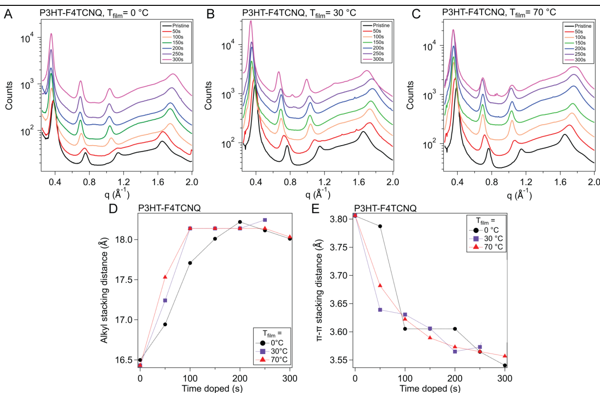
Figure 5. Evolution of ordered structures over the course of doping. Grazing incidence wide angle x-ray scattering (GIWAXS) was conducted on P3HT vapor doped with F4TCNQ at 50 s intervals from 0 s to 300 s for all three sample temperatures. (A), (B), and (C) show the azimuthal linecuts of the scattering images, such as the ones seen in Figure S10. (D) shows the evolution of the alkyl-stacking spacing, which are represented in the linecuts as the first three, equal spaced out peaks. (E) shows the \pi - \pi stacking, which is represented by the broad peak originating around 1.6 \text{ \AA}^{-1} in the neat film.
