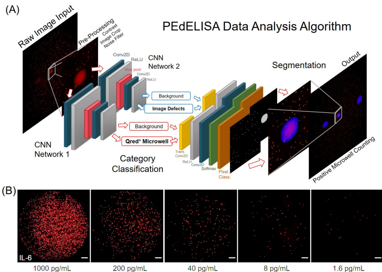
Figure 2. (A) Architecture of the PEdELISA data analysis algorithm using convolutional neural network (CNN) and parallel computing by MATLAB. Two CNN networks were trained and executed in parallel to read in the QuantaRed™ (Qred) fluorescence microwell images, and sequentially performed image pre-processing (including image cropping, contrast enhancement, and noise filtering), category classification, image segmentation, and post-processing (image overlay, visualization, defect compensation, microwell counting). (B) Representative snapshot images of enzyme active “On” microwells on a biosensing pattern (66,724 wells/biosensor) for various analyte concentrations of IL-6. For clear visualization, images of 3600×3600 pixels were cropped from original raw images of 6000×4000 pixels with 80% brightness enhancement and 80% contrast enhancement. All of the scale bars are 200 \mu\text{m} . See Fig. S4 for images taken for IL-1 \beta , TNF- \alpha , IL-10, and IL-6.
