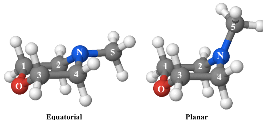
Figure 1. The equatorial and planar structures of NMM.
