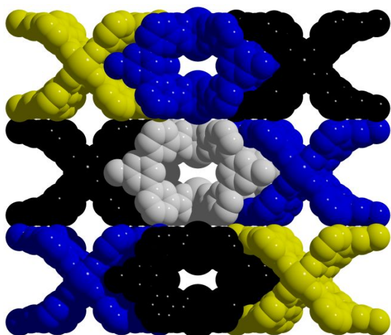
Fig. 2 Solid-state packing of \text{Mo}_4(\text{tdb})_4 where cages in a given layer alternate by 90 degrees.
