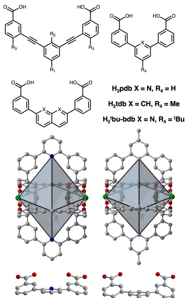
Fig. 1 (Top Left) Prominent ligands for porous lantern-type paddlewheel cages that have been combined with Cu, Mo, or Rh to afford M_4L_4 structures. This study focuses on Cu_4(\text{pdb})_4 , Cu_4(\text{'bu-bdb})_4 , and M_4(\text{tdb})_4 where M = \text{Cr, Cu, Mo} . (Bottom) Structures of Cu_4(\text{pdb})_4 (left) and Cu_4(\text{tdb})_4 (right) where green, red, gray, and blue spheres represent copper, oxygen, carbon, and nitrogen atoms, respectively. Although the pyridine-based cage has no C-H on the central ring, the ligand is significantly distorted away from planarity in the crystal structure.
