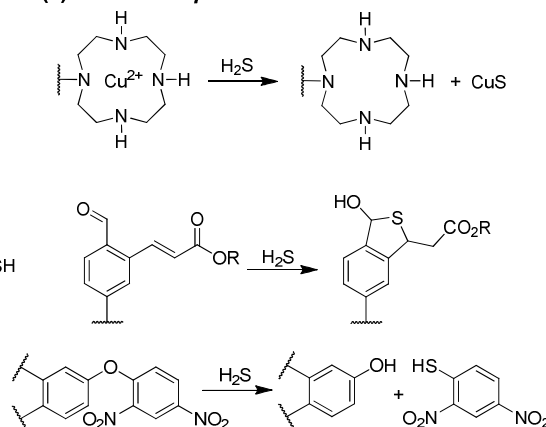
Scheme 4. Common motifs in reaction-based probes for H 2 S, including reactions based on (a) reduction, (b) nucleophilic attack, and (c) metal precipitation.
