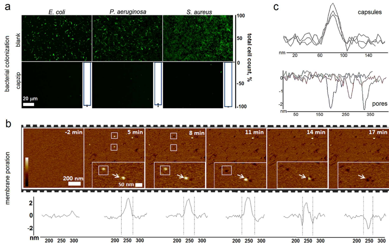
Fig. 5 Capzip-promoted antimicrobial activity and mechanism. (a) Confocal micrographs of bacterial cells after 16-hour incubations with and without capzip, stained with membrane-permeant SYTO ® 9. White histogram bars denote total cell counts (%) for bacterial colonization with capzip after subtracting background adhesion taken as 100%. (b) AFM topography of SLBs during capzip incubation in solution. White boxes and arrows highlight individual capsule conversions into pores. Color scale is 6 nm. Cross sections show the evolution of a capsule (white arrow in inset images) into a pore in real time. (c) Representative cross-sections of capsules and pores.
