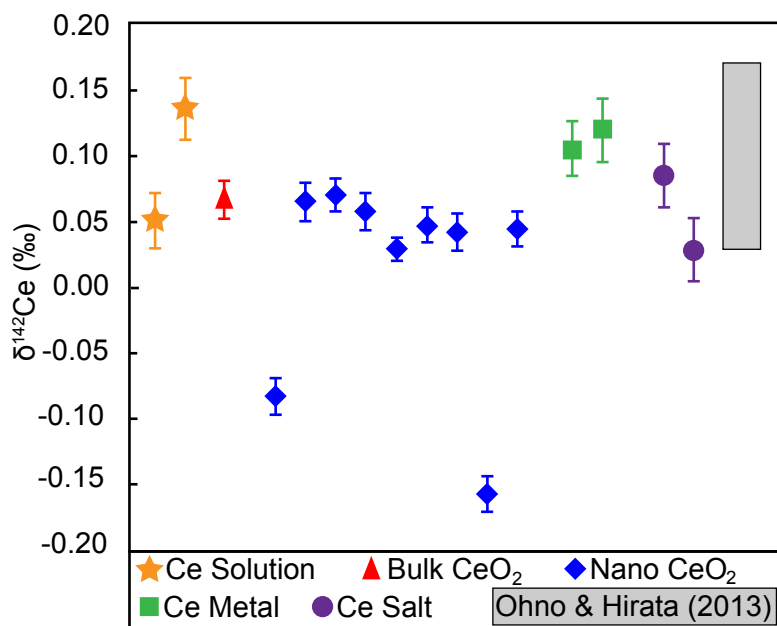
Figure 3 \delta^{142}\text{Ce} data for the Ce samples analysed in this study. Error bars denote the 2 \sigma uncertainties that were calculated based on multiple analyses ( n = 5 to 15; Table 1). The grey field denotes the range of \delta^{142}\text{Ce} values determined by Ohno and Hirata 6 for 5 rock samples. However, the position of this field in relation to our data may not be accurate, as a different Ce reference material were applied to define \delta^{142}\text{Ce} = 0 .
