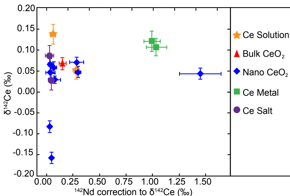
Figure 1 The \delta^{142}\text{Ce} values of the purified Ce materials (Table 1) are plotted against the correction to the \delta^{142}\text{Ce} values for the presence of isobaric ^{142}\text{Nd} (Table 3). The error bars associated with the x-axis denote the range of corrections applied to the \delta^{142}\text{Ce} values for the presence of isobaric ^{142}\text{Nd} (Table 3), whereas the y-axis error bars denote the 2se uncertainties of the \delta^{142}\text{Ce} values based on multiple analyses ( n = 5 to 15; Table 1).
