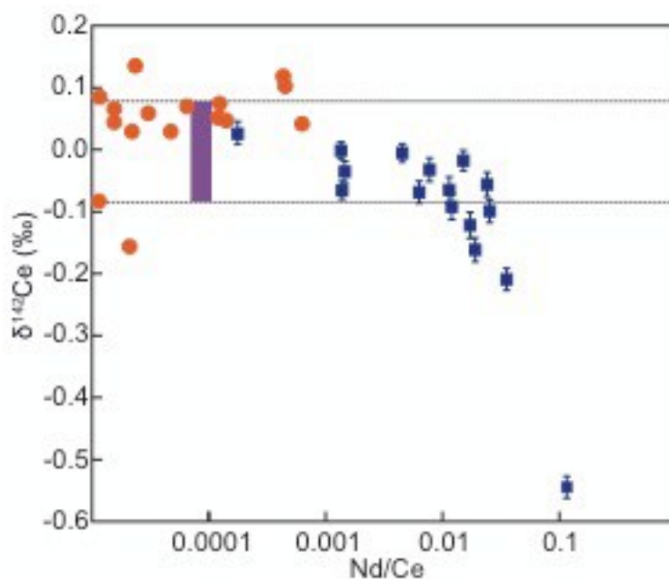
Figure 2 Plot of measured \delta^{142}\text{Ce} values versus the Nd/Ce ratios of the sample solutions. The purple bar and dotted lines denote the 2sd uncertainty determined from multiple analyses of the Alfa Aesar Ce standard solution ( \pm 0.09\text{‰} , n = 25 ). The data obtained for Alfa Aesar Ce standard solutions doped with varying levels of Nd (blue squares with internal 2sd uncertainties) demonstrate that accurate \delta^{142}\text{Ce} values can be readily obtained at Nd/Ce ratios of up to 0.01. The orange circles represent the Ce samples that were analysed in this study.
