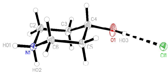
Figure 6. The formula unit of hydrochloride 2 in the crystal. Ellipsoids correspond to 50% probability levels.
