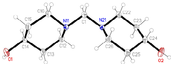
Figure 6. The formula unit of hydrochloride 2 in the crystal. Ellipsoids correspond to 50% probability levels.
