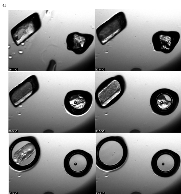
Figure 13. Microscopic images at various temperatures (36.1, 87.5, 90.5, 91.5, 92.5, 93.5°C) obtained by thermomicroscopy with form 1t (crystal on left) and form 1o (crystal on right).
