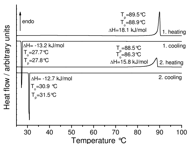
Figure 9. DSC heating and cooling curves for form 1 at 1°C/min; the peak ( T_p ) and onset ( T_o ) temperatures are given in °C and the enthalpy \Delta H in kJ/mol.
