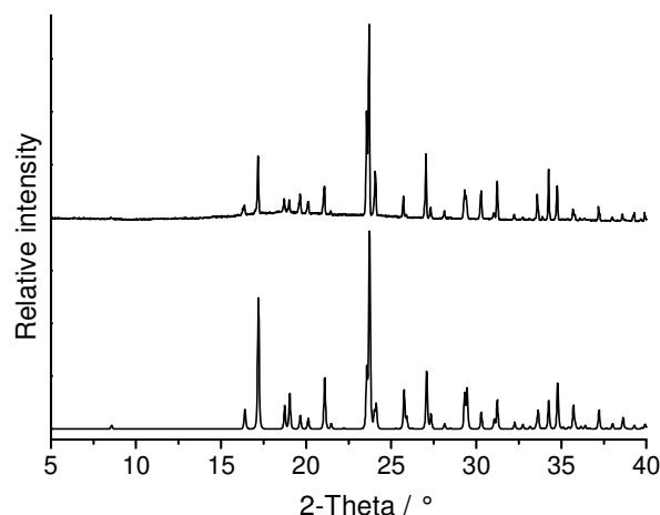
Figure 12. Experimental X-ray powder pattern of the residue obtained from dichloromethane (top) and calculated powder pattern for the hydrochloride 2 (bottom).
