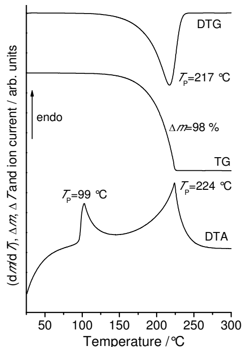
Figure 11. DTA, TG and DTG curve for form 1t at 4°C/min in a nitrogen atmosphere
