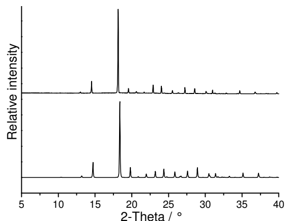
Figure 10. Experimental X-ray powder pattern of the solidified melt of form 1t (top) and calculated powder pattern for form 1t (bottom).
