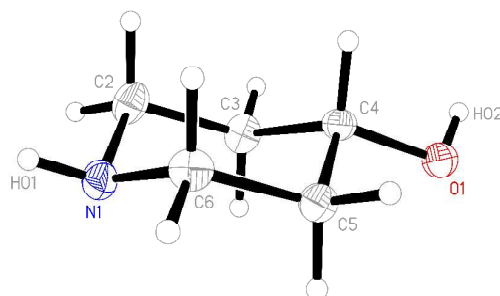
Figure 4. The molecule of 1o in the crystal. Ellipsoids correspond to 50% probability levels.
