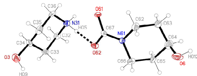
Figure 8. One of three independent formula units of carbamate 4 in the crystal. Ellipsoids correspond to 50% probability levels. The dashed line represents a classical hydrogen bond.
