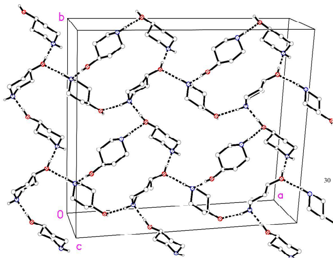
Figure 5. Packing diagram of 10 with view direction perpendicular to the plane (111). Classical hydrogen bonds are drawn as thick dashed lines. The two types of helical chain mentioned in the text run horizontally (two chains) and vertically (three chains).
