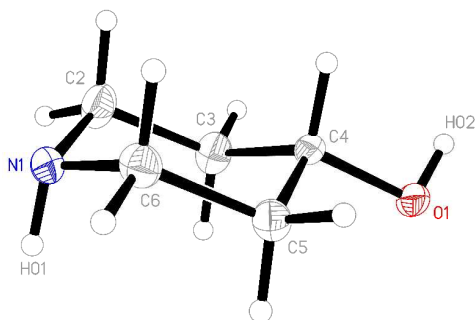
Figure 2. The molecule of 1t in the crystal. Ellipsoids correspond to 50% probability levels.
