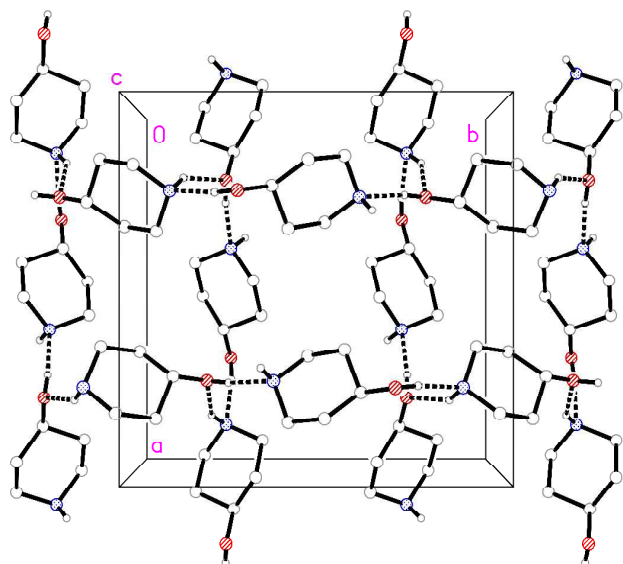
Figure 3. Packing diagram of 1t with view direction parallel to the c axis. Classical hydrogen bonds are drawn as thick dashed lines. Nitrogen atoms are drawn blue and oxygens red.
