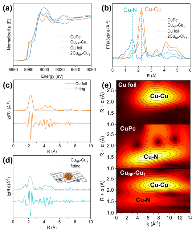
Fig. 2 (a) Cu K-edge XANES spectra of \text{Cu}_{\text{NP}}\text{-Cu}_1 and 2\text{Cu}_{\text{NP}}\text{-Cu}_1 , in comparison to Cu foil and CuPc. (b) Fourier-transform (FT)-EXAFS spectra of \text{Cu}_{\text{NP}}\text{-Cu}_1 , 2\text{Cu}_{\text{NP}}\text{-Cu}_1 , Cu foil and CuPc. FT-EXAFS spectral fittings for (c) Cu foil and (d) the \text{Cu}_{\text{NP}}\text{-Cu}_1 catalyst. (e) Wavelet-transform (WT)-EXAFS of \text{Cu}_{\text{NP}}\text{-Cu}_1 , CuPc and Cu foil at the Cu K-edge.
