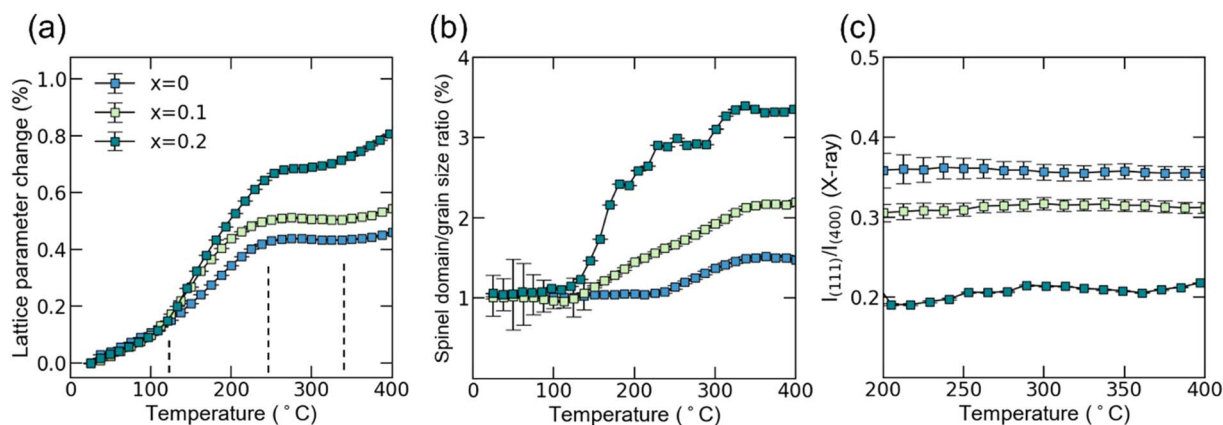
Fig. 6 Monitoring the thermally-induced structural transformation in \text{Li}_{0.5}\text{Mn}_{0.7}\text{Zr}_{0.2-x}\text{Ti}_x\text{O}_2 ( x = 0, 0.1, \text{ and } 0.2 ) compounds using SXR with in situ heating from room temperature to 400 °C ((a)–(c)). (a) A lattice parameter evolution, (b) ratio of the average spinel domain size to the average grain size, and (c) ratio of the (111) peak intensity ( I_{(111)} ) to the (400) peak intensity ( I_{(400)} ) upon heating. The I_{(111)}/I_{(400)} ratio is indicative of the relative occupancy of the 16c and 16d octahedral sites.
