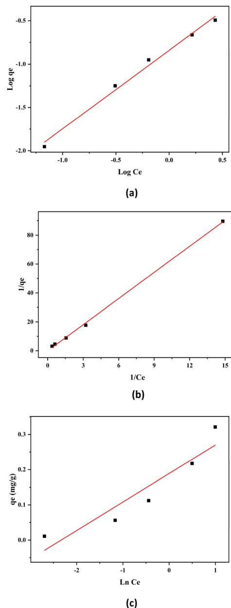
Fig. 13 (a) The Freundlich isotherm illustrating the adsorption of \text{Pb(II)} onto AOR–PVA–CH composite blends, (b) the Langmuir isotherm illustrating the adsorption of \text{Pb(II)} onto AOR–PVA–CH composite blends, and (c) the Temkin isotherm illustrating the adsorption of \text{Pb(II)} onto AOR–PVA–CH composite blends.
